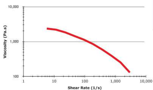
Shear-Viscosity @ 190 °C
